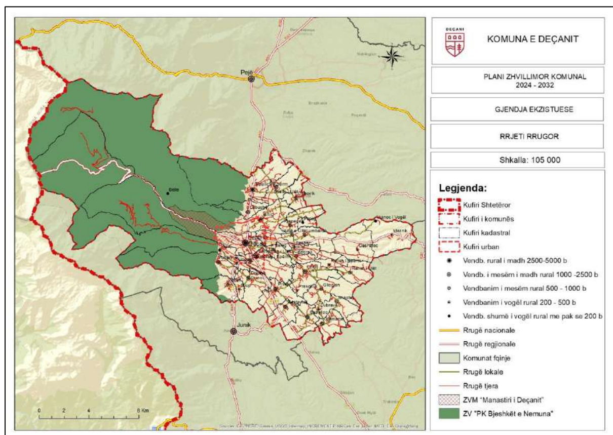
Harta 15 Rrjeti rrugor
